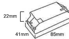
model no. : GFN-TFLMVC8A Drive, INPUT : 100-240V MAX : 6W (350mA)
