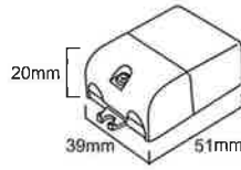
model no. : GFN-TFLSVC3AZ / GFN-TFLSVC3BZ Drive, INPUT : 100-240V MAX : 3W (350mA) / 3W x 1 (700mA)
